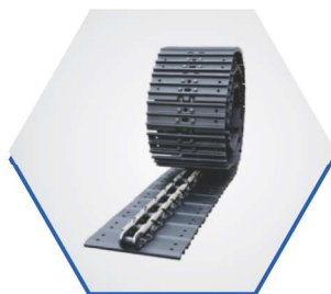
Track Group
